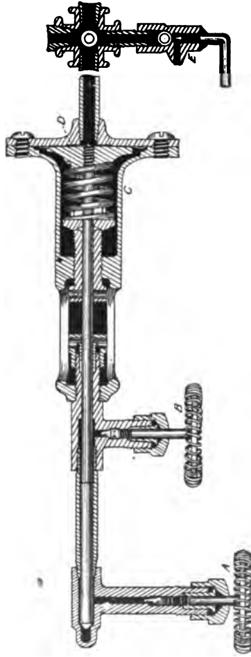
FIG. 97. —Fuel Feed Regulator of a Steam Carriage Burner, intended for use with "Torch" Burner Kindler or Auxiliary Vaporizer. A is the hand wheel and needle valve regulating the feed to the main burner; B, the hand wheel and valve for operating the torch; C, the spring and header attached to the main valve rod; D, the diaphragm against which steam bears, regulating the main valve according to pressure; E, the drip valve for condensed steam on the steam inlet to diaphragm. The liquid gasoline is admitted at a port on the left-hand extremity of the regulator tube, near the end of the needle valve on the main rod.
